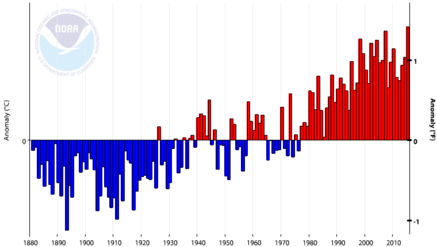
Global Land and Ocean Temperature Anomalies, December-February
